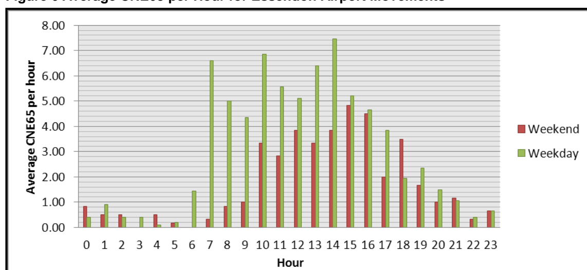
Figure 6 Average CNE65 per Hour for Essendon Airport Movements
