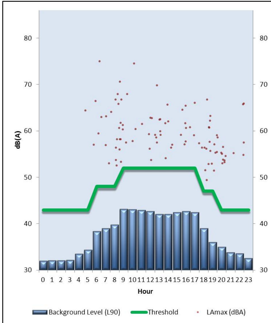
FIGURE 1: ROLEYSTONE NOISE SUMMARY 31/03/2014 12:00AM – 28/04/2014 12:00AM
