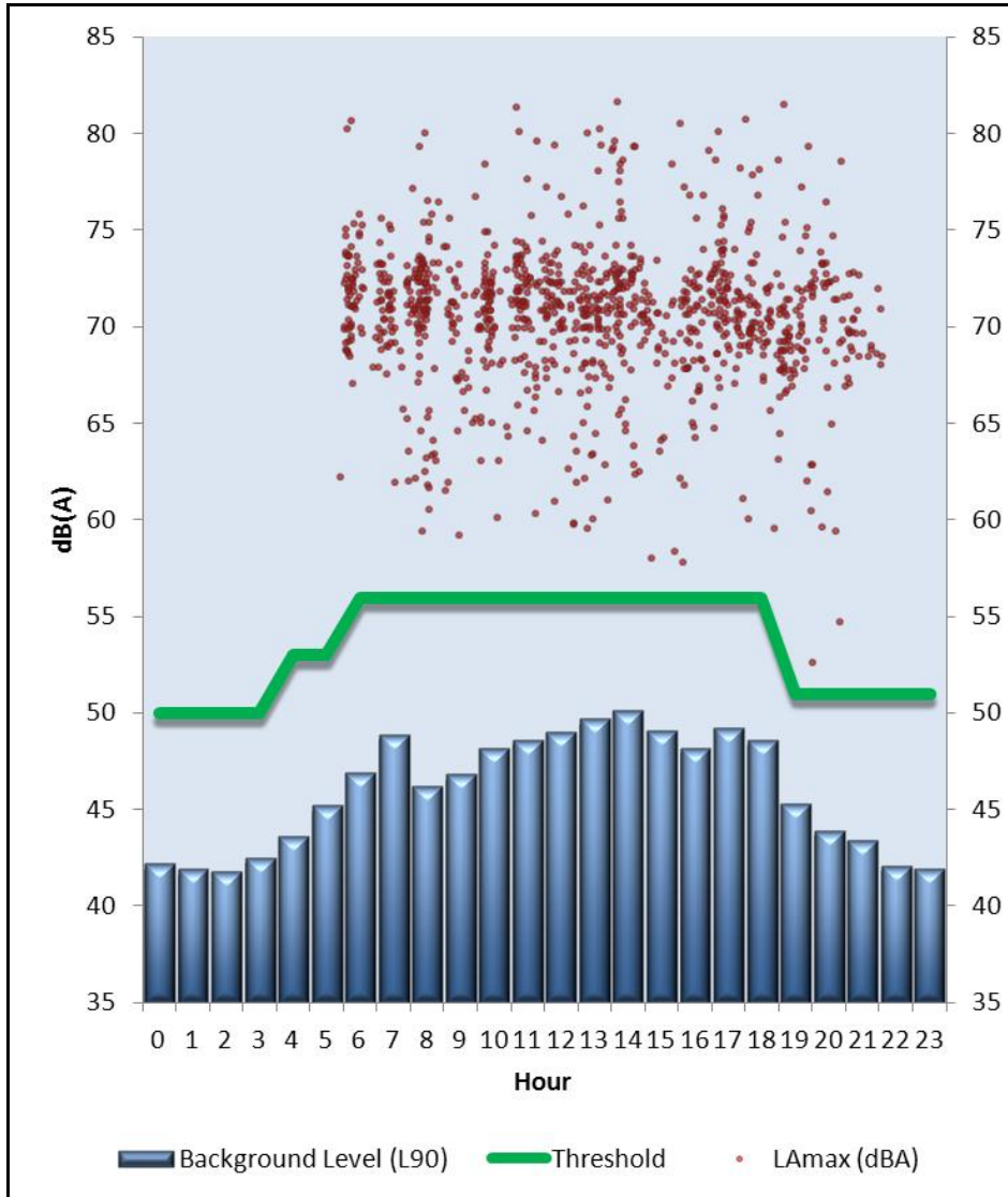
FIGURE 1: OXLEY COVE NOISE SUMMARY 03/02/2014 12:00AM – 03/03/2014 12:00AM
