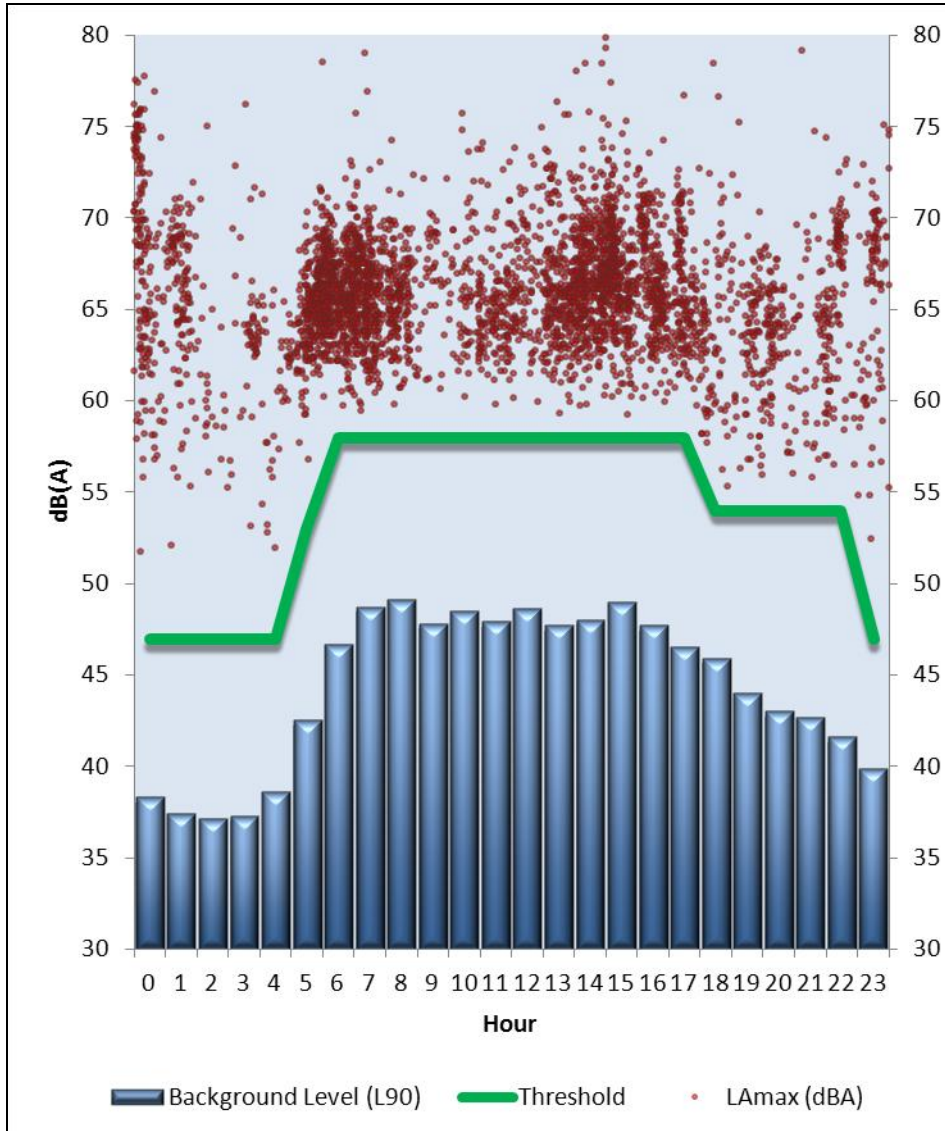
FIGURE 1: MANNING NOISE SUMMARY 07/07/2014 12:00AM – 29/09/2014 12:00AM
